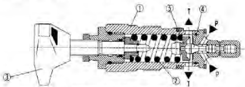
DBDH...K...10B/...(poppet valve)
