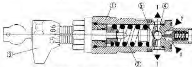
DBDA...K...10B/...(ball valve)
